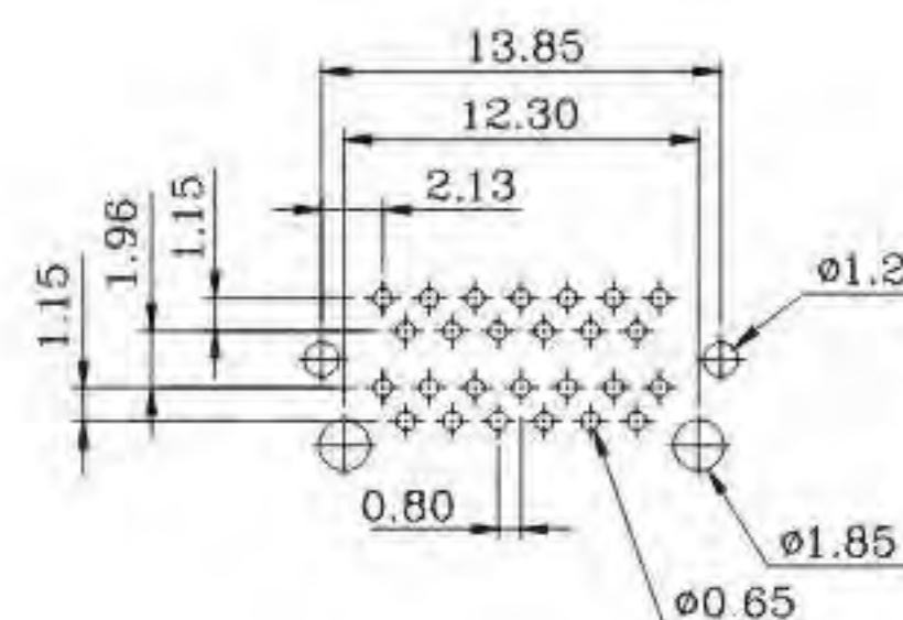
PCB Layout
